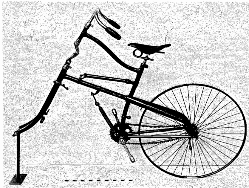
Figure 14 Whippet spring frame (1885). Photograph courtesy of the Trustees of the Science Museum, London.
