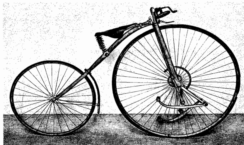
Figure 16 Geared Facile bicycle (1888). Photograph courtesy of the Trustees of the Science Museum, London.
